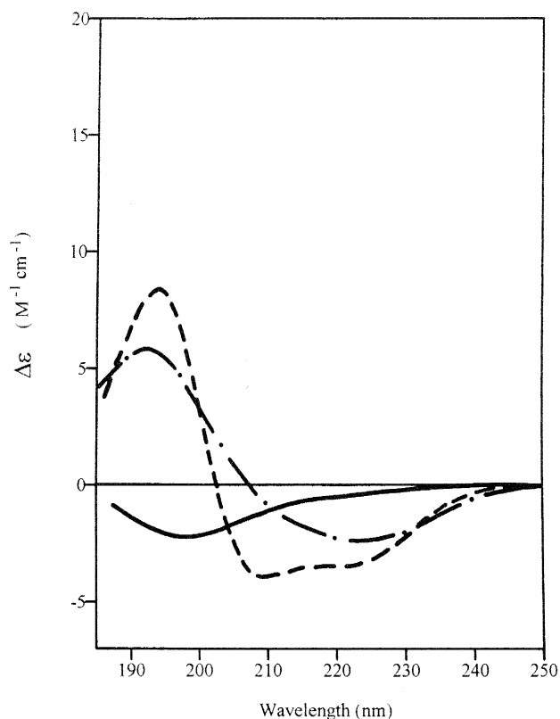
Fig. 2. The CD spectra of P4, P5 and P6 in aqueous solution. CD was used to determine the structures of P4 (solid line), P5 dashed line) and P6 (dash-dotted line) in aqueous solution, at their intrinsic pH. For 0.1 mM P5, this pH was measured as pH 4.1 and the peptide readily adopted an \alpha -helical conformation which constituted 29% of the P5 structure. By contrast, P6 was sparingly soluble, exhibiting a \beta -strand structure typical of aggregation whereas 0.1 mM P4 was found to possess an intrinsic pH of 4.4 and demonstrated an irregular structure.
